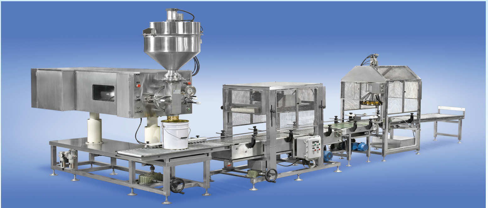
AF MODEL PVF SERIES SOLVENT BASED (EX-PROOF) VOLUMETRIC TIN/PAIL FILLING LINE
